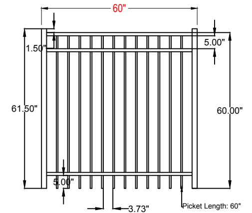
Mode: C02-A-G5X5 Flat Top 3 Rail Gate 5'x5'
