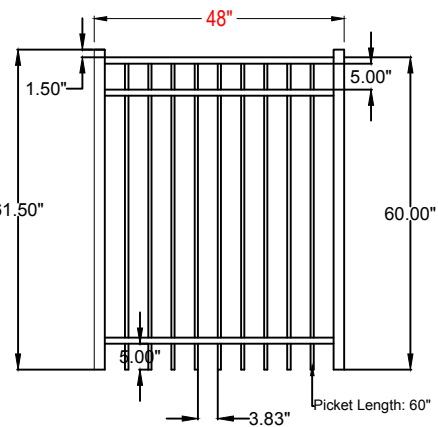
Mode: C02-A-G5X4 Flat Top 3 Rail Gate 5'x4'
