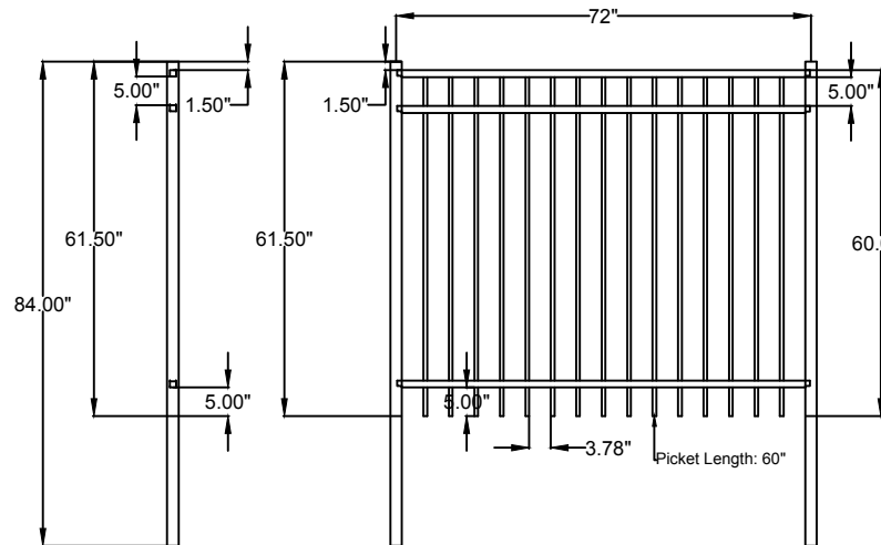
Model: C02-A-5X6 Ornamental Alu Pool Fence 3 Rail Des: 5ftx6ft
